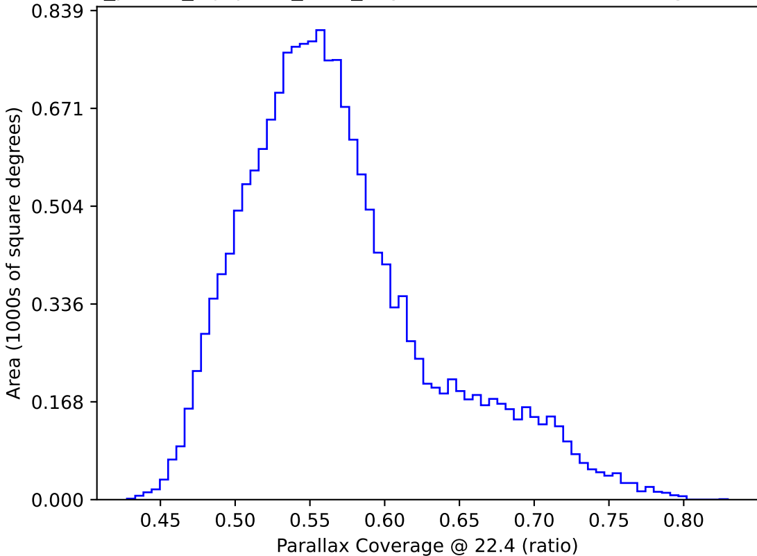
roll_pause_mjdp120_v3.4_10yrs WFD: Parallax Coverage @ 22.4
