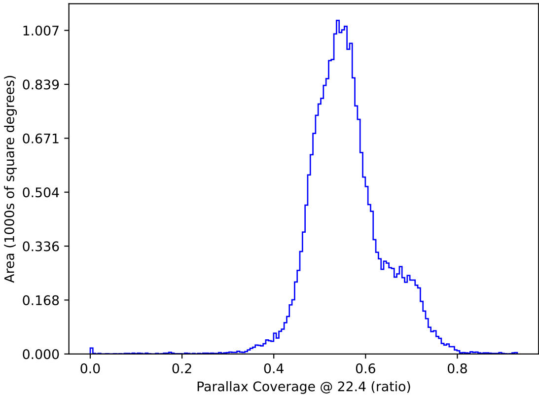
roll_pause_mjdp120_v3.4_10yrs All sky: Parallax Coverage @ 22.4
