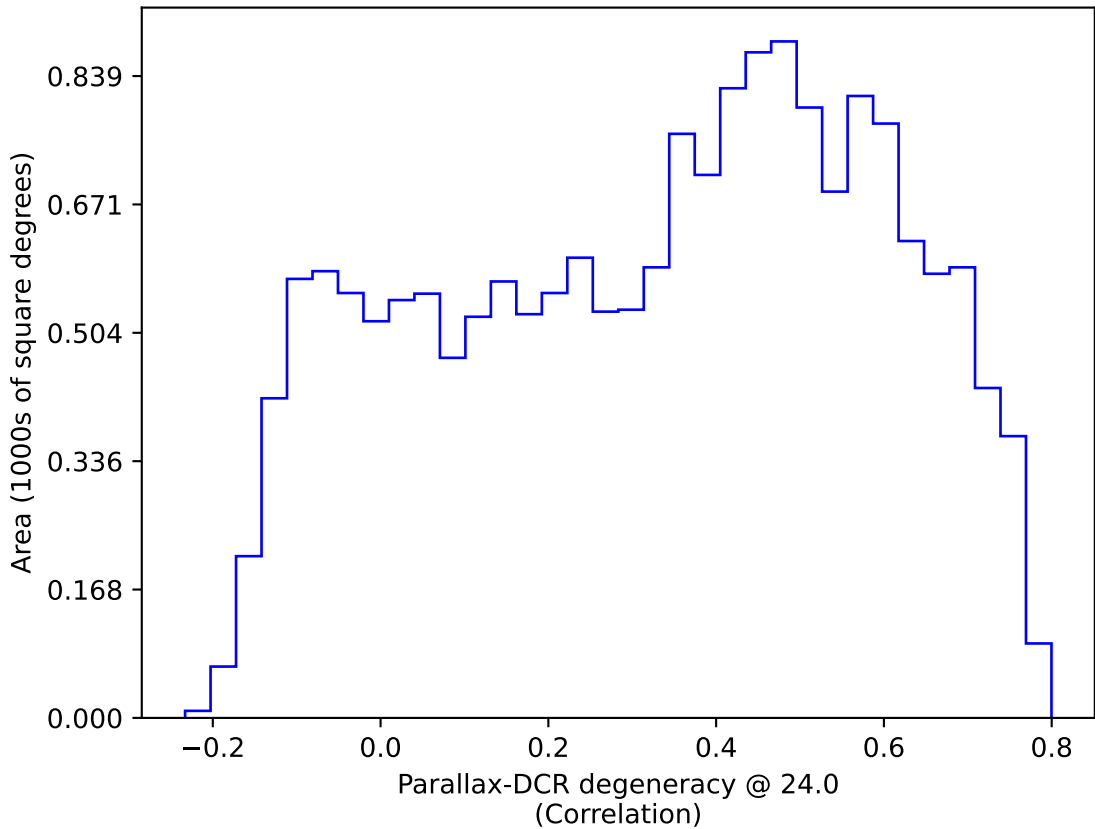
roll_pause_mjdp120_v3.4_10yrs WFD: Parallax-DCR degeneracy @ 24.0
