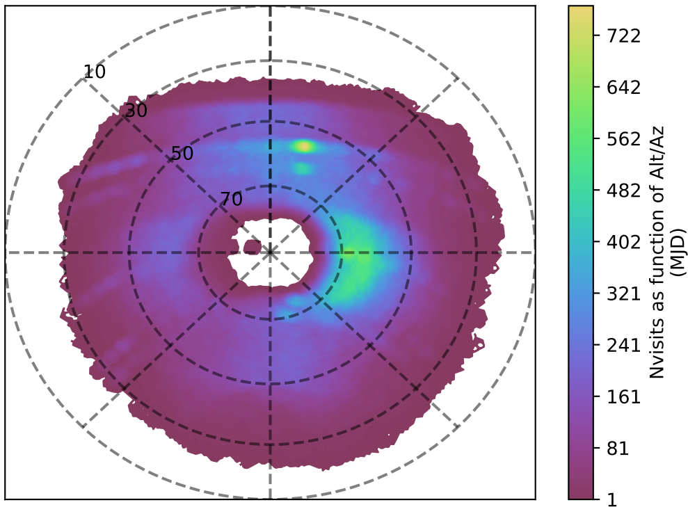
roll_pause_mjdp120_v3.4_10yrs u band: Nvisits as function of Alt/Az
