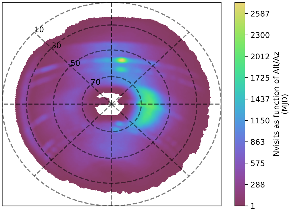
roll_pause_mjdp120_v3.4_10yrs r band: Nvisits as function of Alt/Az
