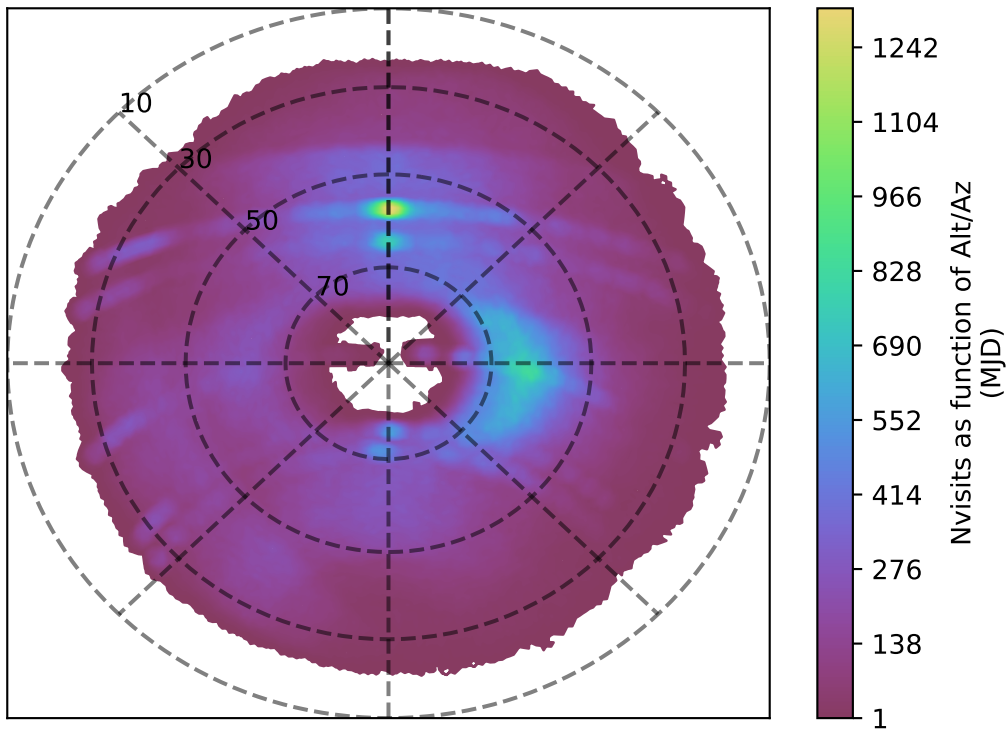
roll_pause_mjdp120_v3.4_10yrs g band: Nvisits as function of Alt/Az
