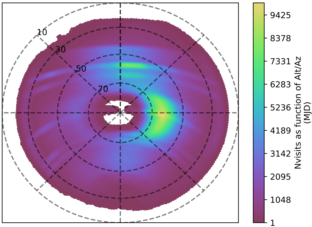
roll_pause_mjdp120_v3.4_10yrs all bands: Nvisits as function of Alt/Az
