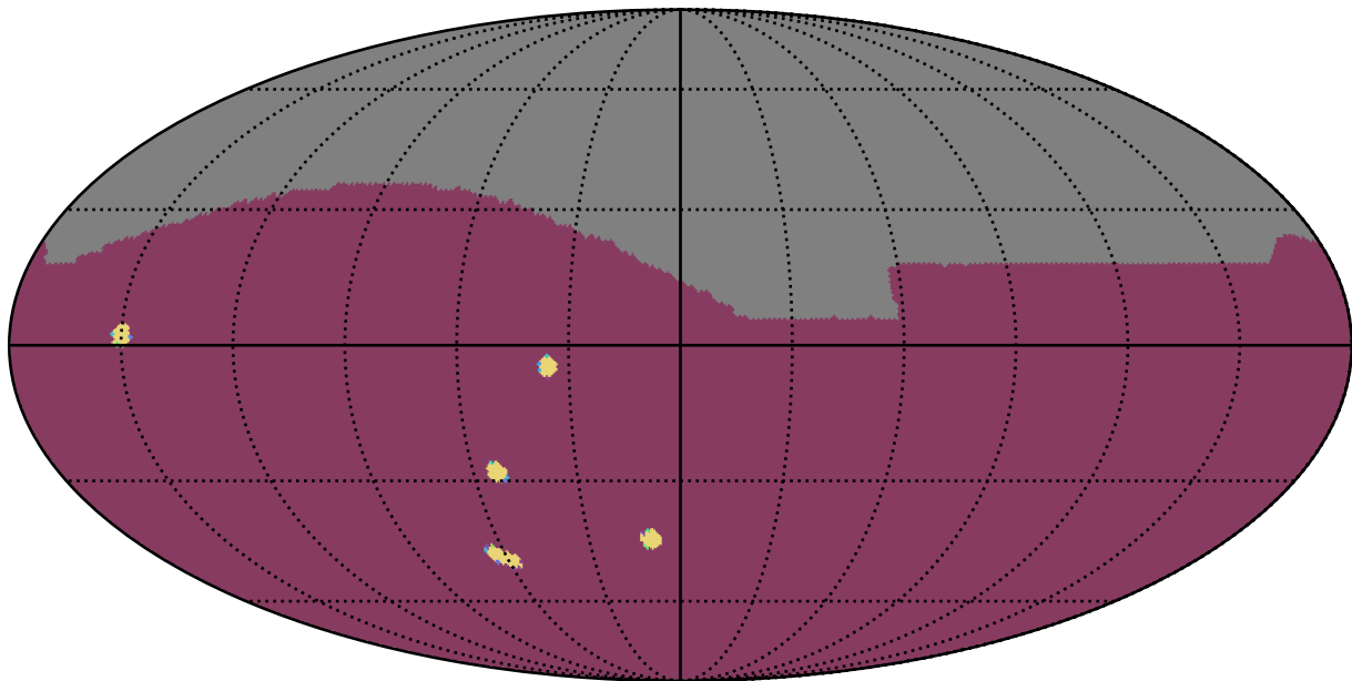
roll_pause_mjdp120_v3.4_10yrs All sky: NumberOfQuickRevisits
