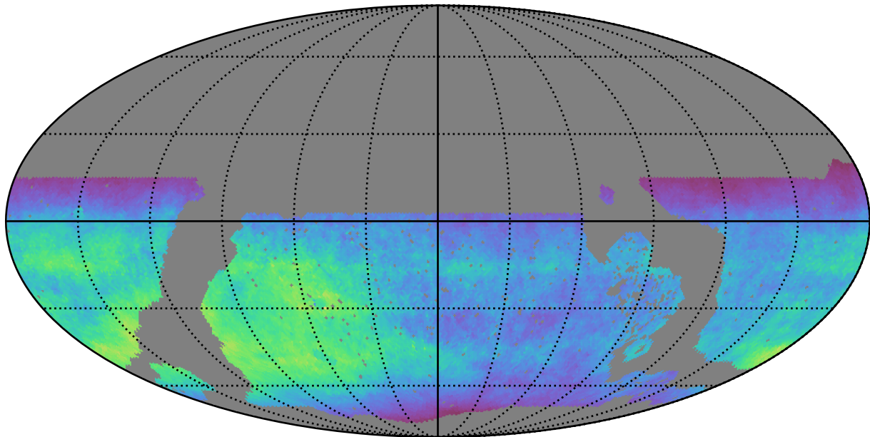
roll_pause_mjdp120_v3.4_10yrs WFD z band: Normalized Teff
