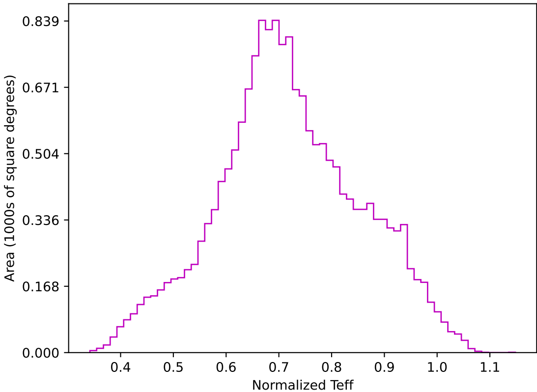
roll_pause_mjdp120_v3.4_10yrs WFD z band: Normalized Teff
