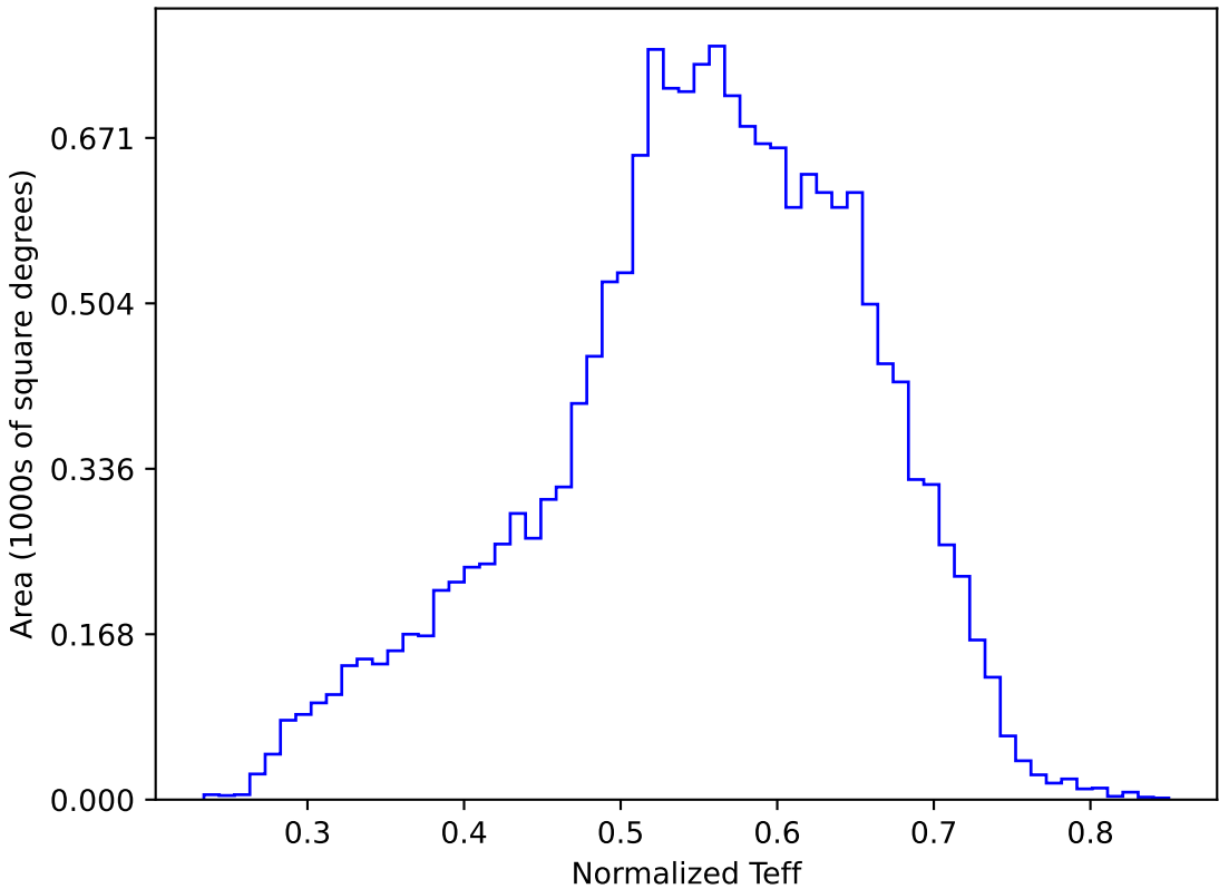
roll_pause_mjdp120_v3.4_10yrs WFD y band: Normalized Teff
