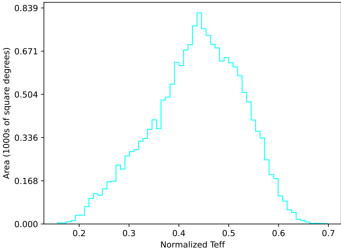
roll_pause_mjdp120_v3.4_10yrs WFD u band: Normalized Teff
