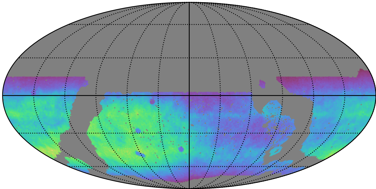
roll_pause_mjdp120_v3.4_10yrs WFD r band: Normalized Teff
