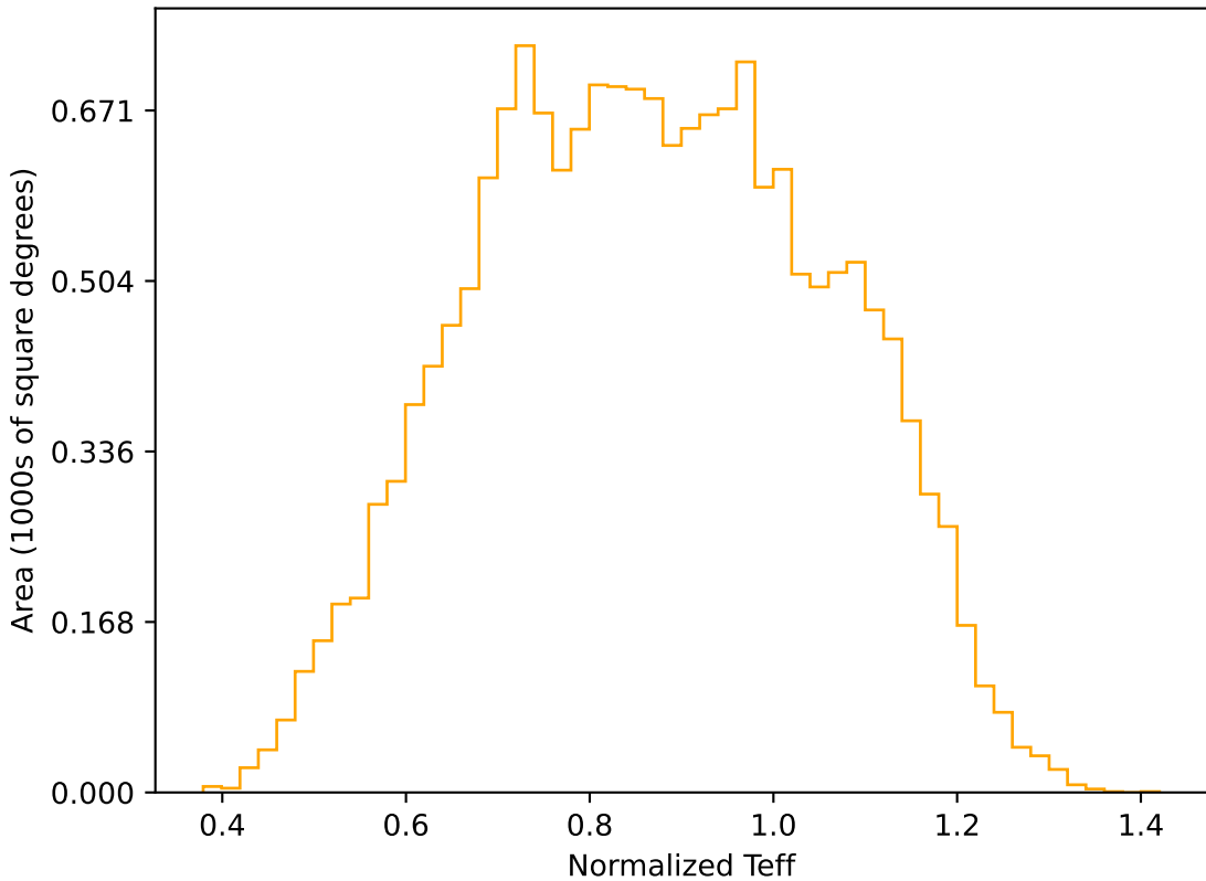
roll_pause_mjdp120_v3.4_10yrs WFD r band: Normalized Teff
