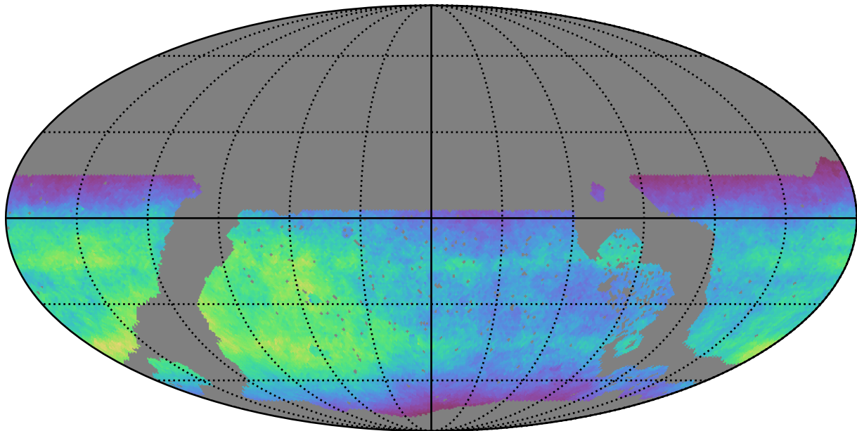
roll_pause_mjdp120_v3.4_10yrs WFD i band: Normalized Teff
