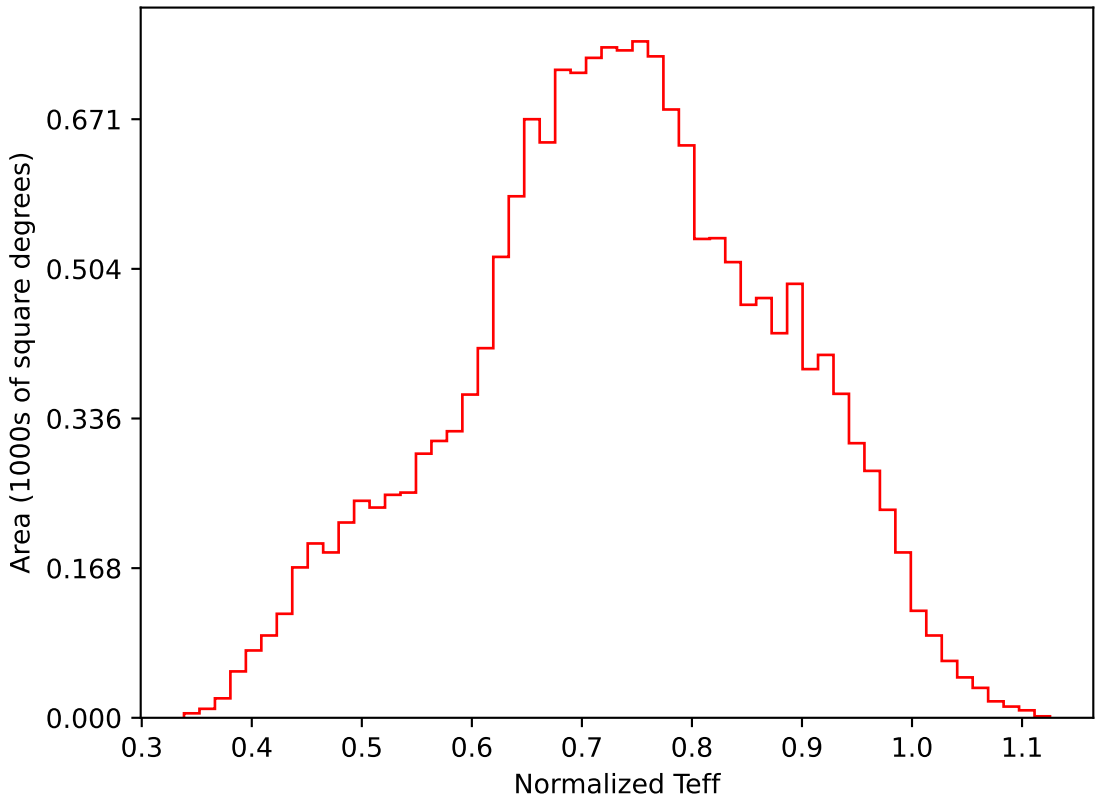
roll_pause_mjdp120_v3.4_10yrs WFD i band: Normalized Teff
