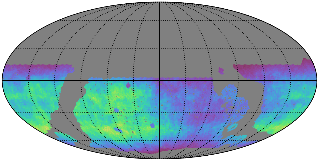
roll_pause_mjdp120_v3.4_10yrs WFD g band: Normalized Teff
