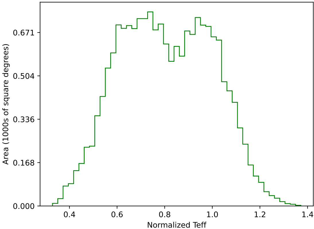
roll_pause_mjdp120_v3.4_10yrs WFD g band: Normalized Teff
