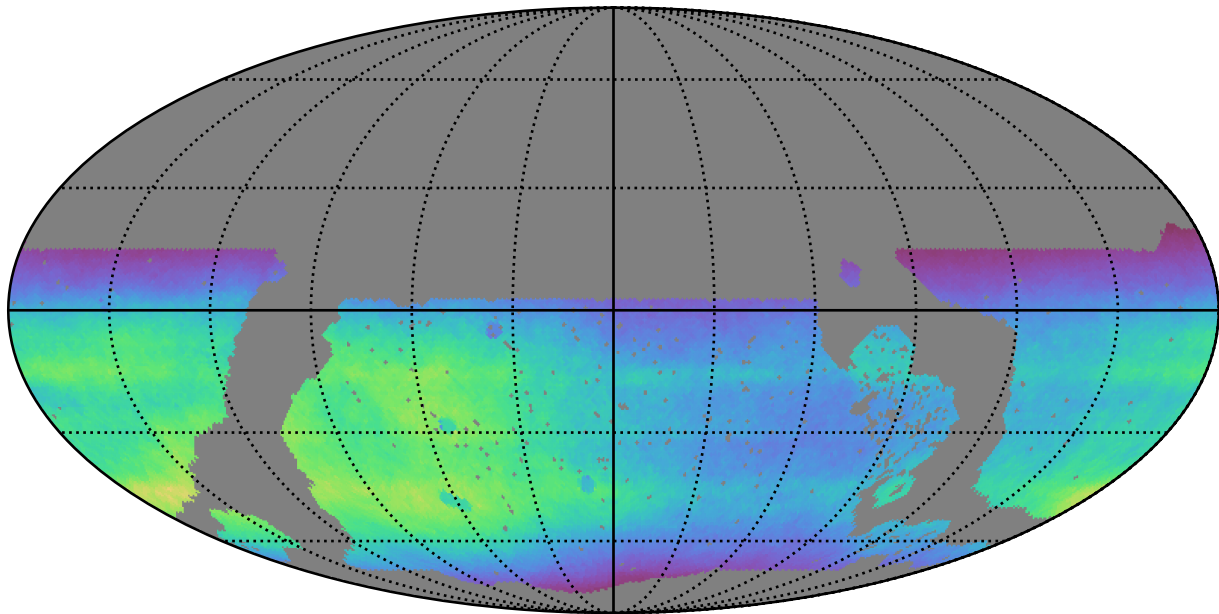
roll_pause_mjdp120_v3.4_10yrs WFD all bands: Normalized Teff
