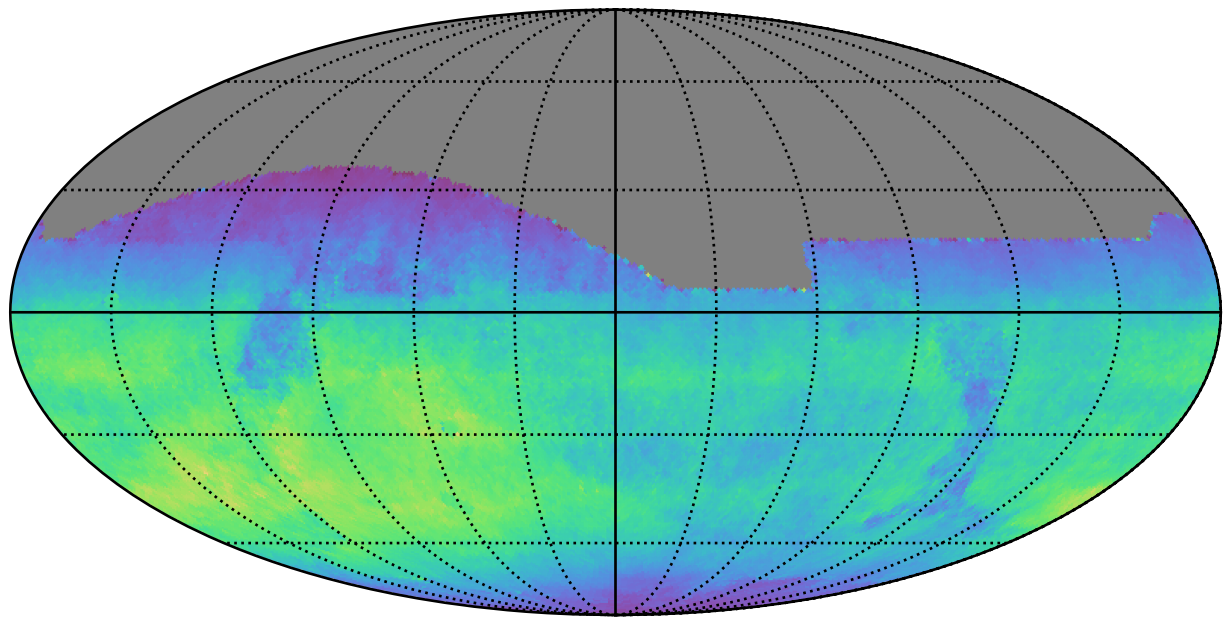
roll_pause_mjdp120_v3.4_10yrs All sky z band: Normalized Teff
