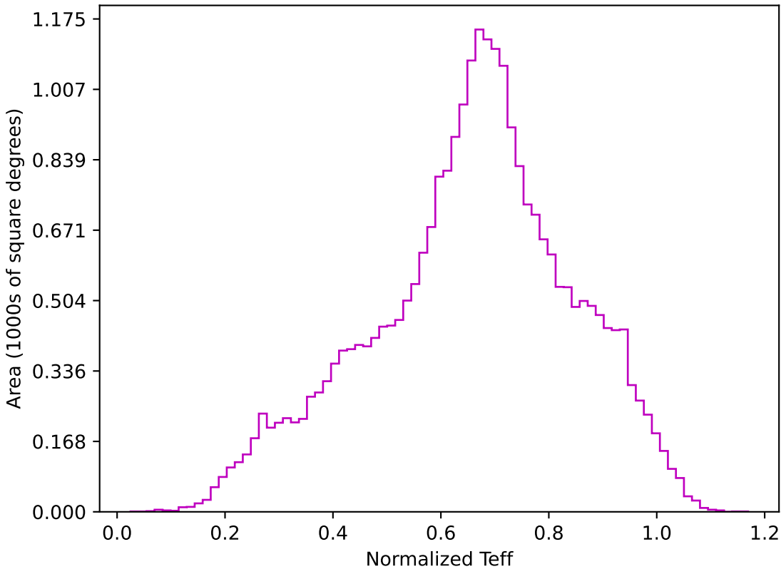
roll_pause_mjdp120_v3.4_10yrs All sky z band: Normalized Teff
