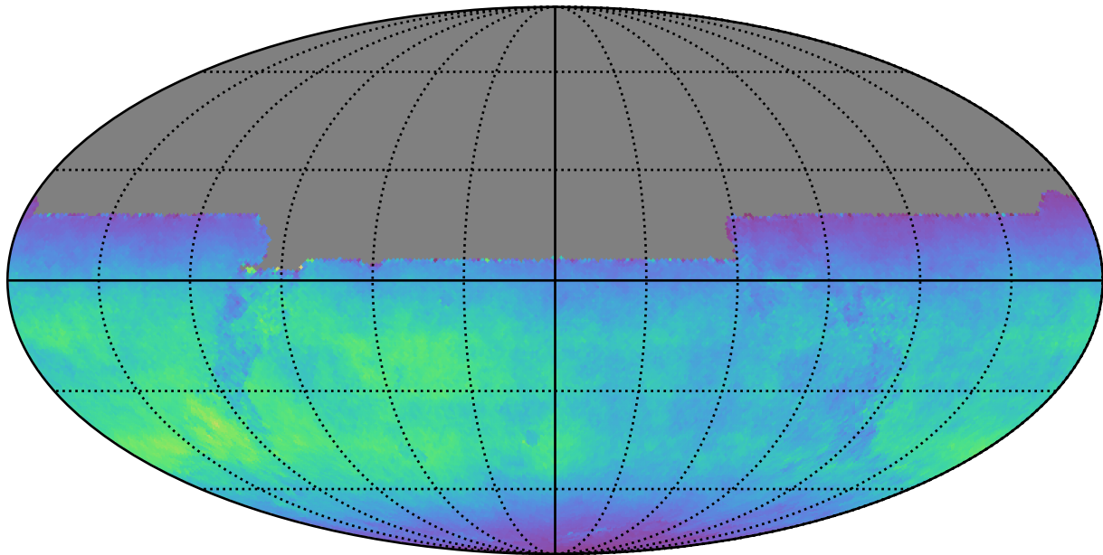
roll_pause_mjdp120_v3.4_10yrs All sky y band: Normalized Teff
