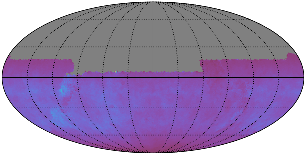
roll_pause_mjdp120_v3.4_10yrs All sky u band: Normalized Teff
