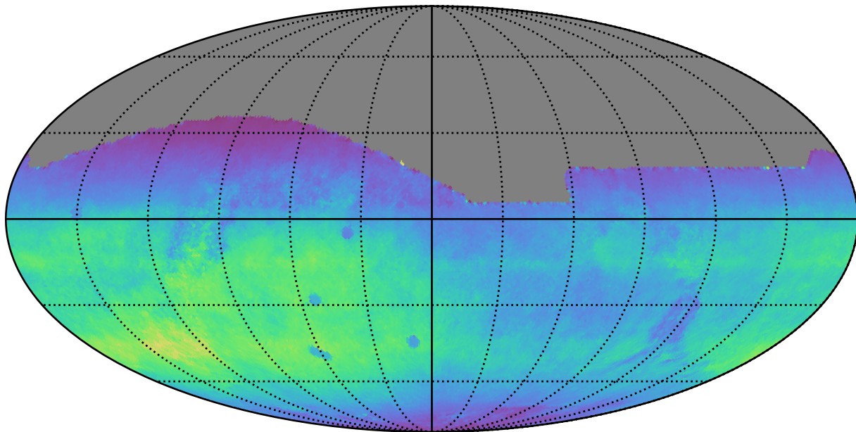
roll_pause_mjdp120_v3.4_10yrs All sky r band: Normalized Teff
