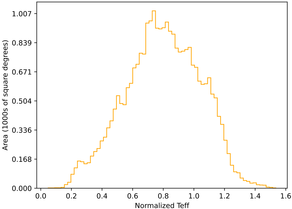
roll_pause_mjdp120_v3.4_10yrs All sky r band: Normalized Teff
