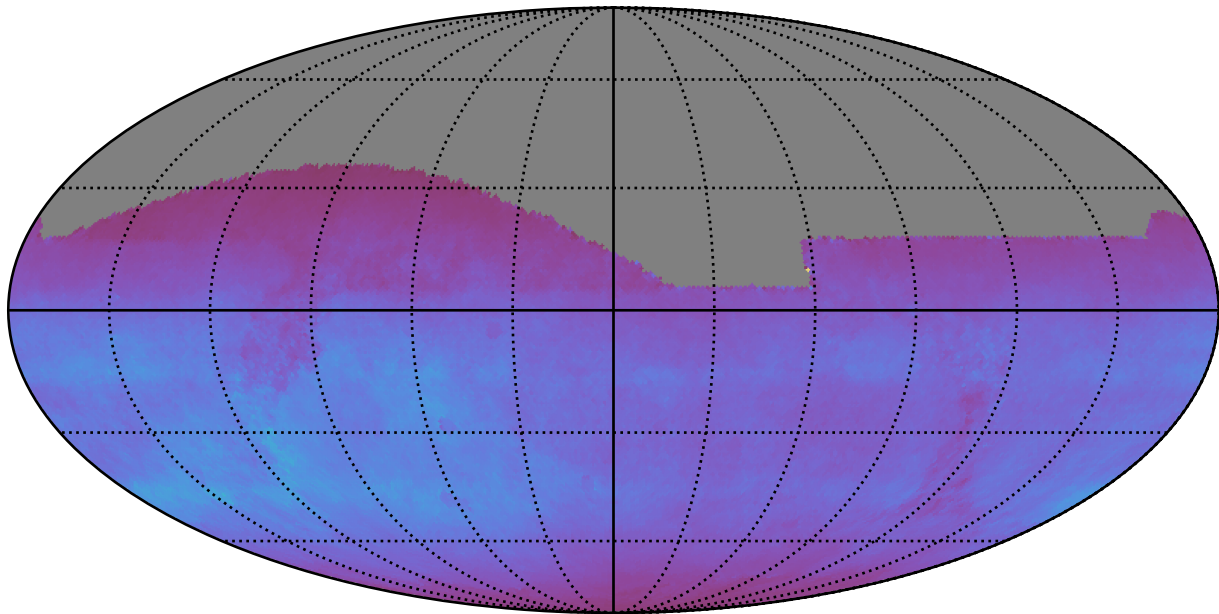
roll_pause_mjdp120_v3.4_10yrs All sky i band: Normalized Teff
