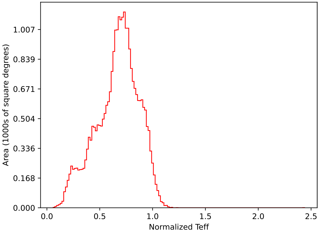
roll_pause_mjdp120_v3.4_10yrs All sky i band: Normalized Teff
