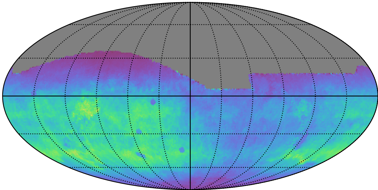
roll_pause_mjdp120_v3.4_10yrs All sky g band: Normalized Teff
