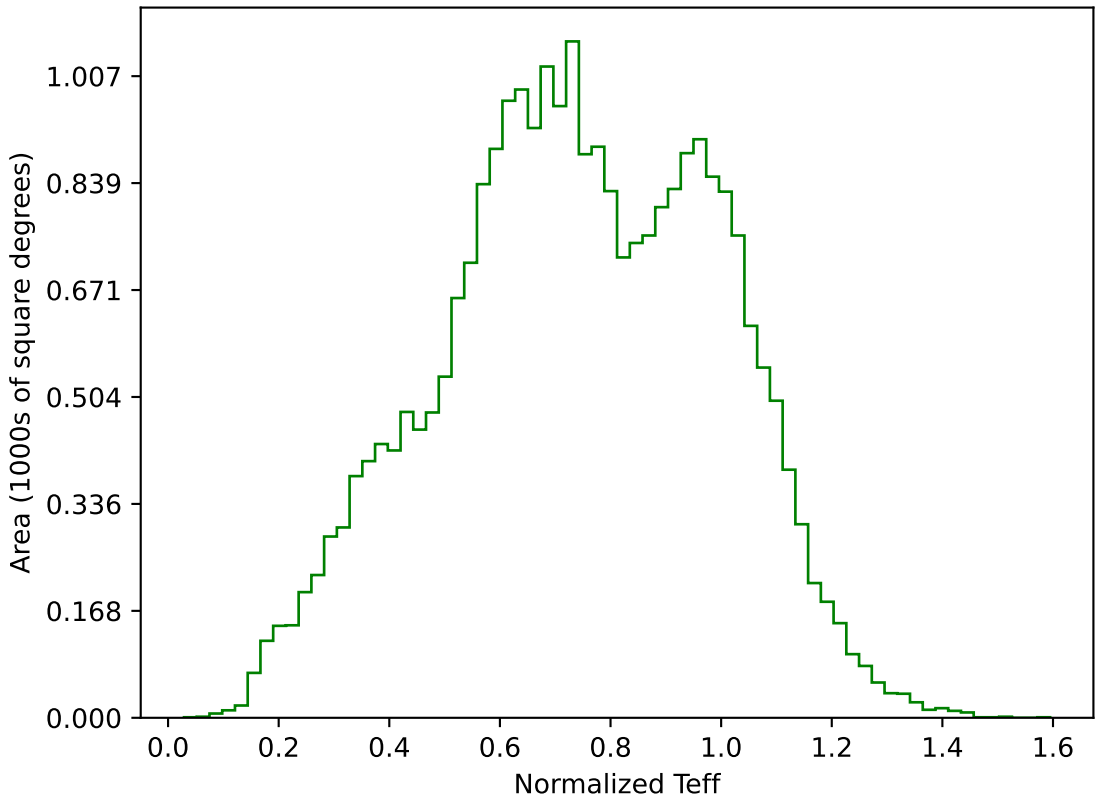
roll_pause_mjdp120_v3.4_10yrs All sky g band: Normalized Teff
