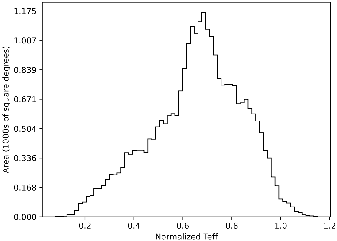
roll_pause_mjdp120_v3.4_10yrs All sky all bands: Normalized Teff
