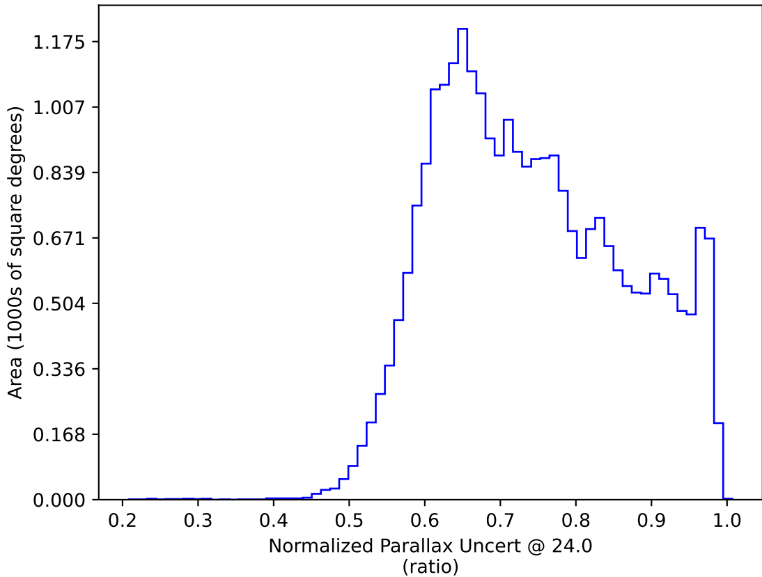
roll_pause_mjdp120_v3.4_10yrs All sky: Normalized Parallax Uncert @ 24.0
