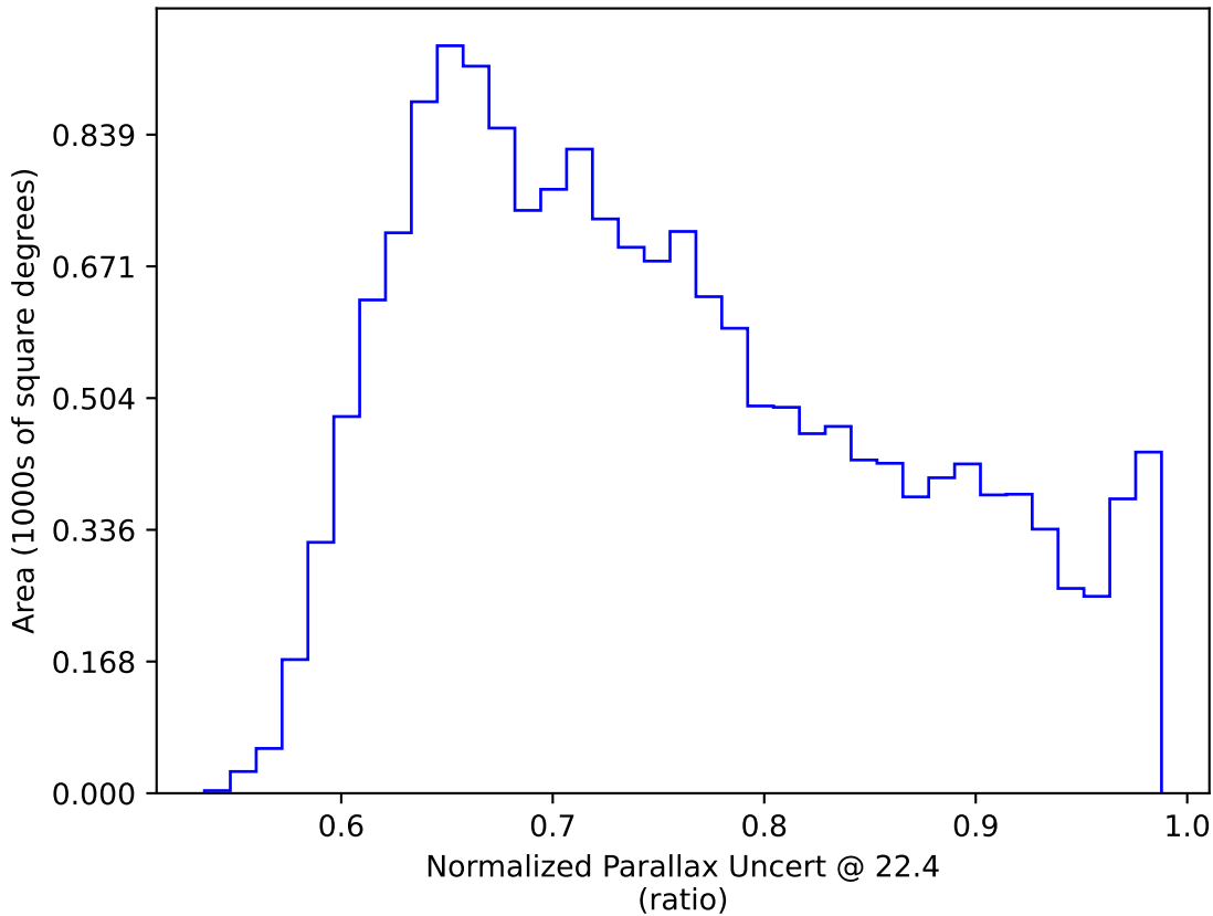
roll_pause_mjdp120_v3.4_10yrs WFD: Normalized Parallax Uncert @ 22.4
