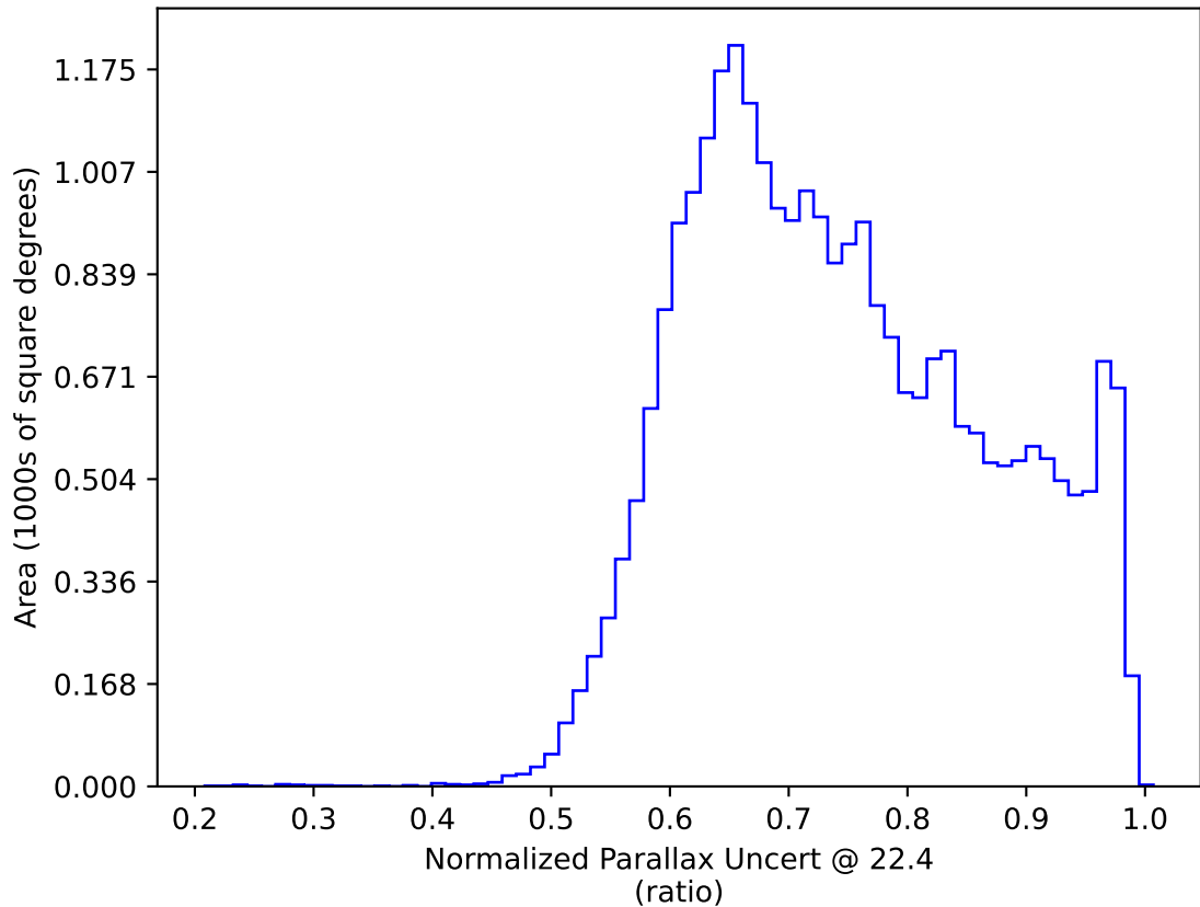
roll_pause_mjdp120_v3.4_10yrs All sky: Normalized Parallax Uncert @ 22.4
