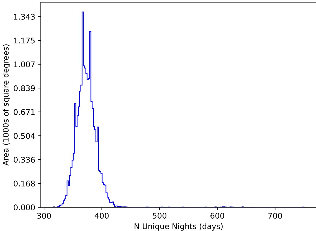
roll_pause_mjdp120_v3.4_10yrs WFD all bands: N Unique Nights
