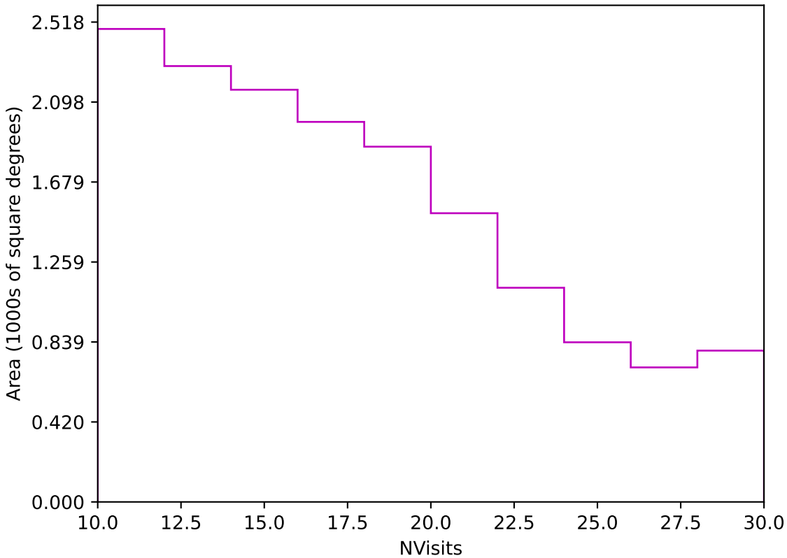
roll_pause_mjdp120_v3.4_10yrs Yr 3-4 z band: NVisits
