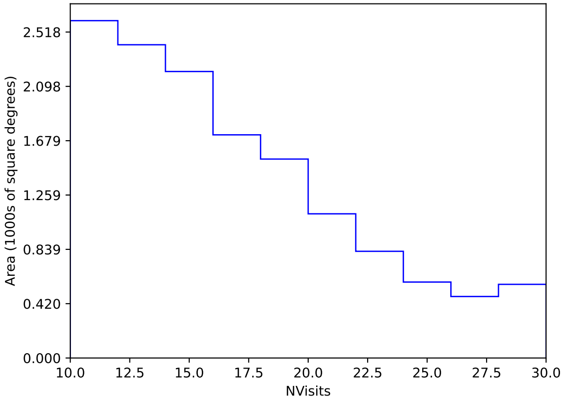
roll_pause_mjdp120_v3.4_10yrs Yr 3-4 y band: NVisits
