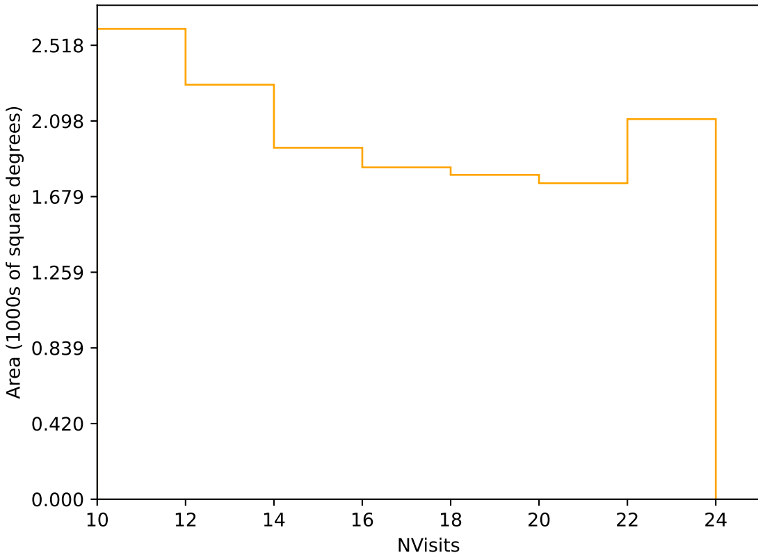
roll_pause_mjdp120_v3.4_10yrs Yr 3-4 r band: NVisits
