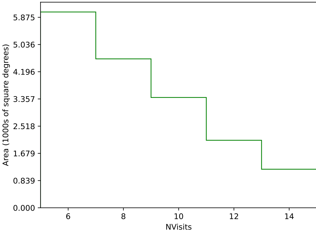
roll_pause_mjdp120_v3.4_10yrs Yr 3-4 g band: NVisits
