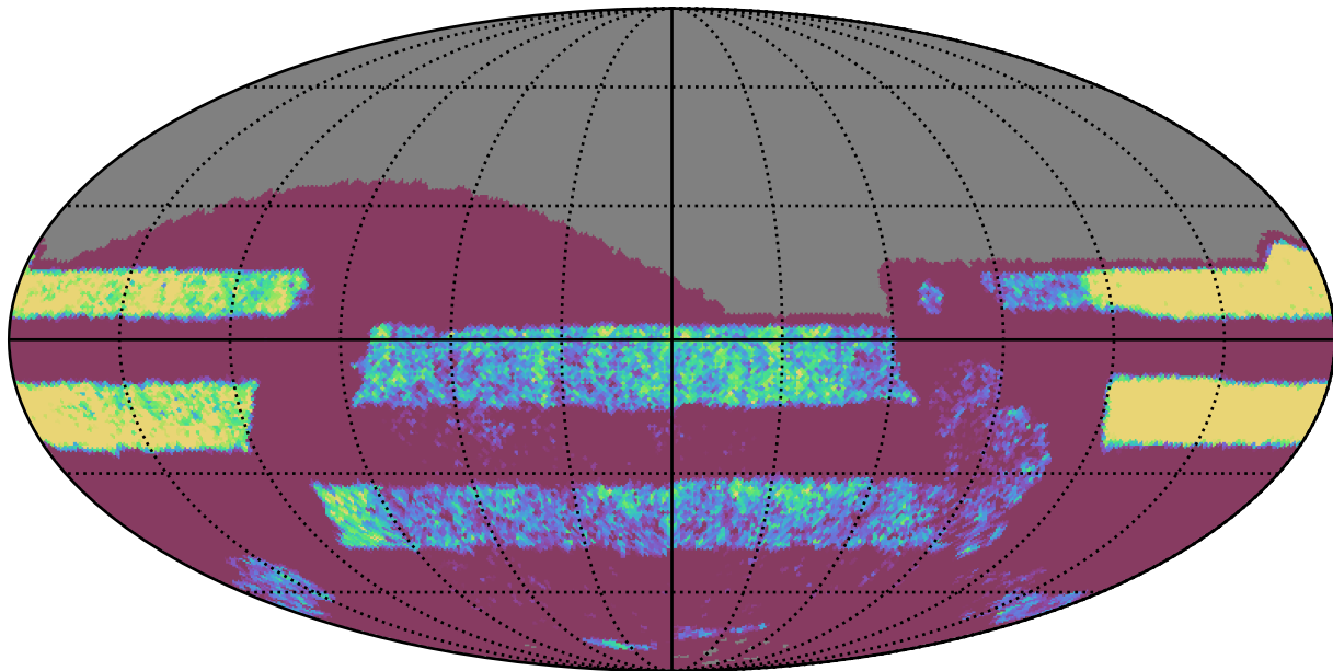
roll_pause_mjdp120_v3.4_10yrs Yr 3-4 all bands: NVisits
