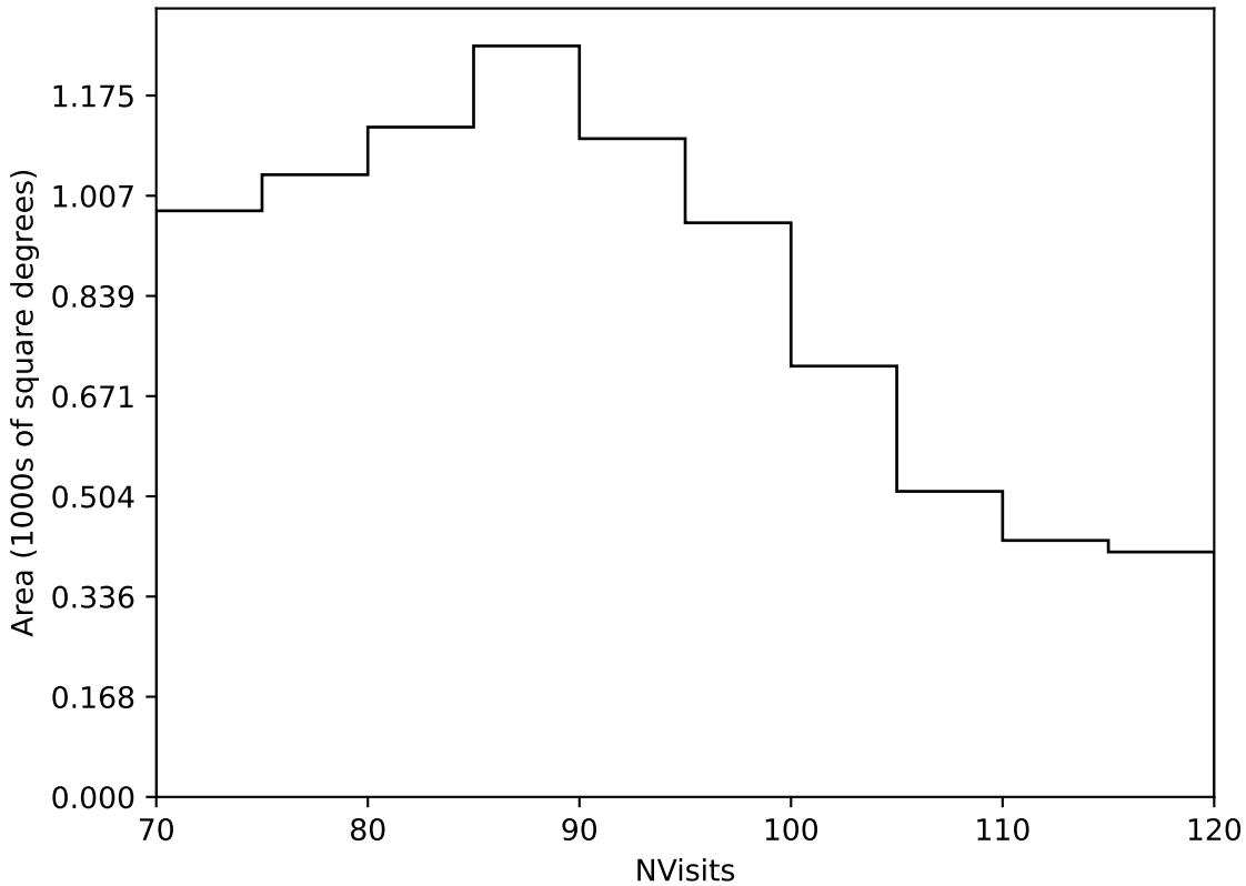
roll_pause_mjdp120_v3.4_10yrs Yr 3-4 all bands: NVisits
