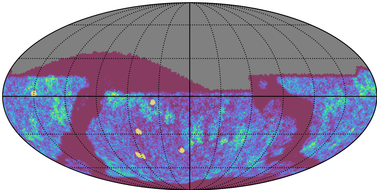
roll_pause_mjdp120_v3.4_10yrs Yr 1 z band: NVisits
