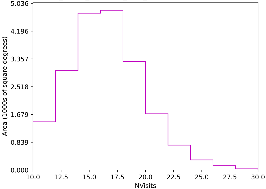
roll_pause_mjdp120_v3.4_10yrs Yr 1 z band: NVisits
