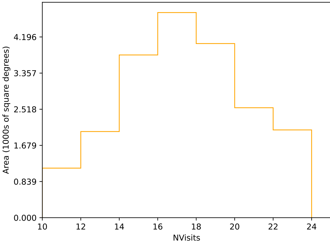
roll_pause_mjdp120_v3.4_10yrs Yr 1 r band: NVisits
