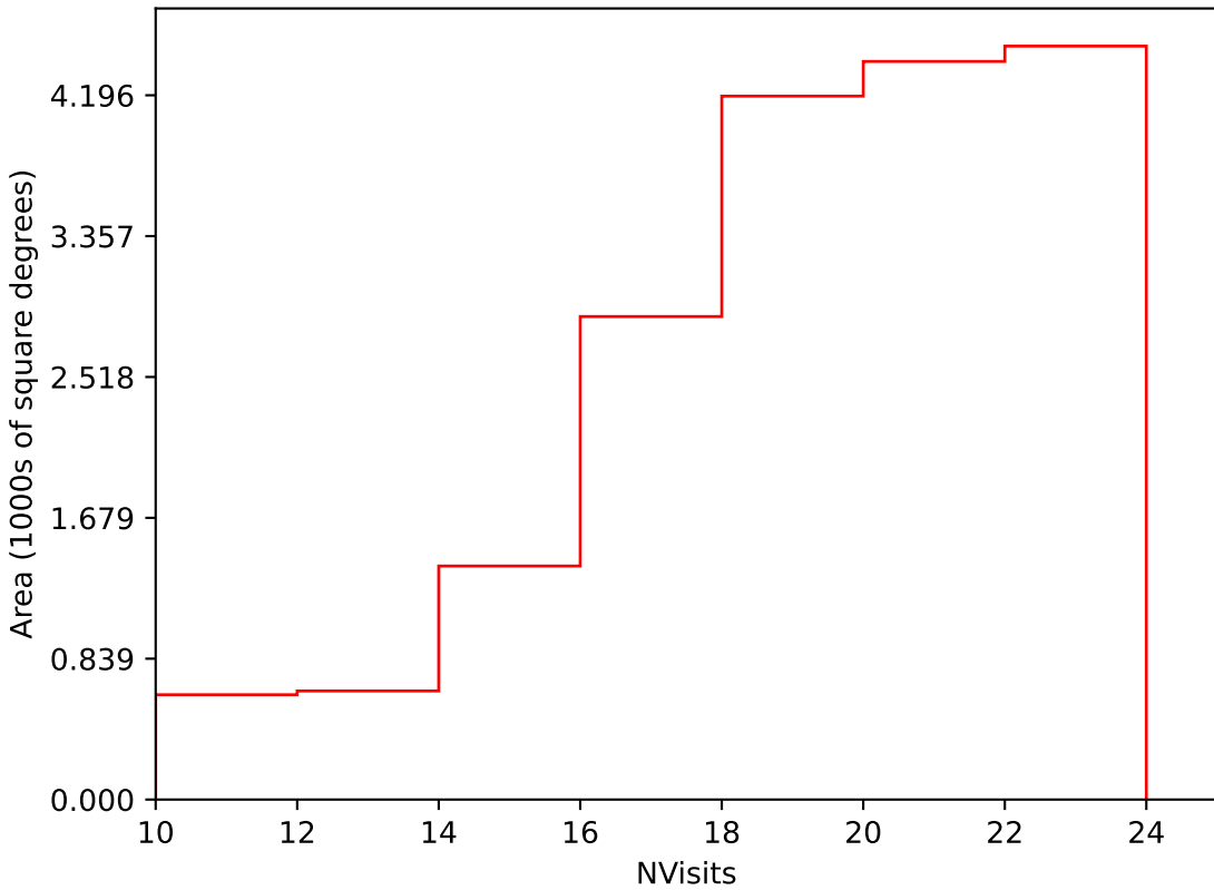
roll_pause_mjdp120_v3.4_10yrs Yr 1 i band: NVisits
