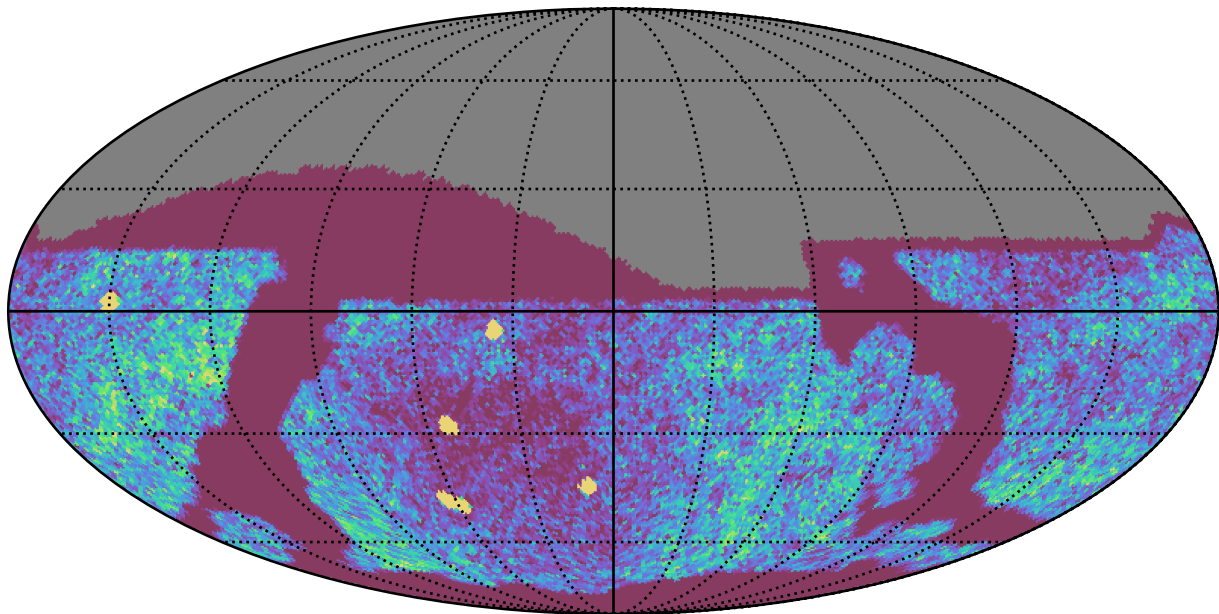
roll_pause_mjdp120_v3.4_10yrs Yr 1 all bands: NVisits
