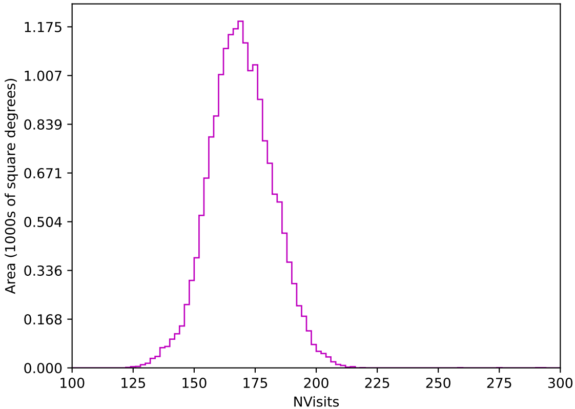
roll_pause_mjdp120_v3.4_10yrs WFD z band: NVisits
