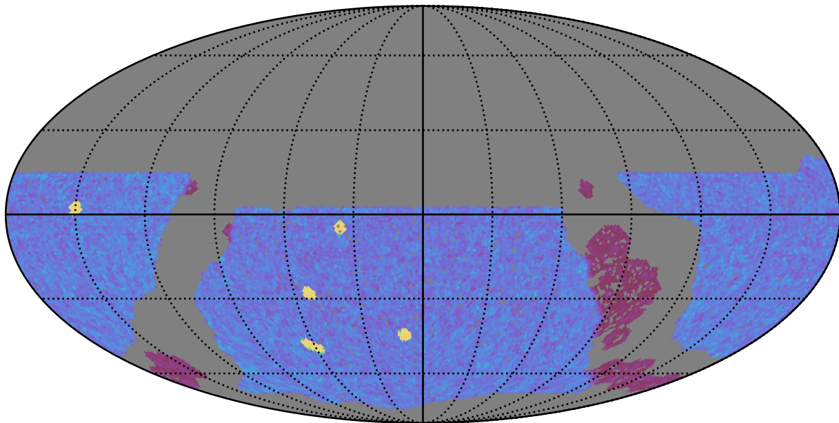
roll_pause_mjdp120_v3.4_10yrs WFD y band: NVisits
