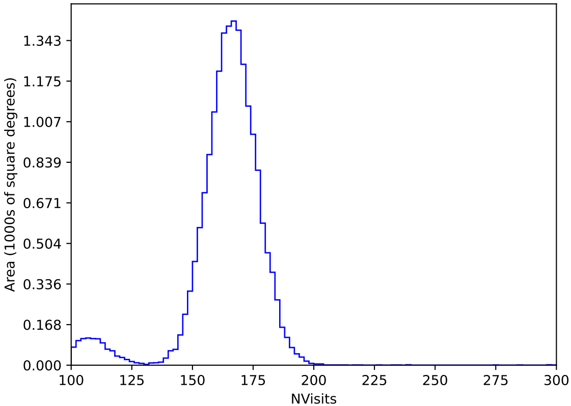
roll_pause_mjdp120_v3.4_10yrs WFD y band: NVisits
