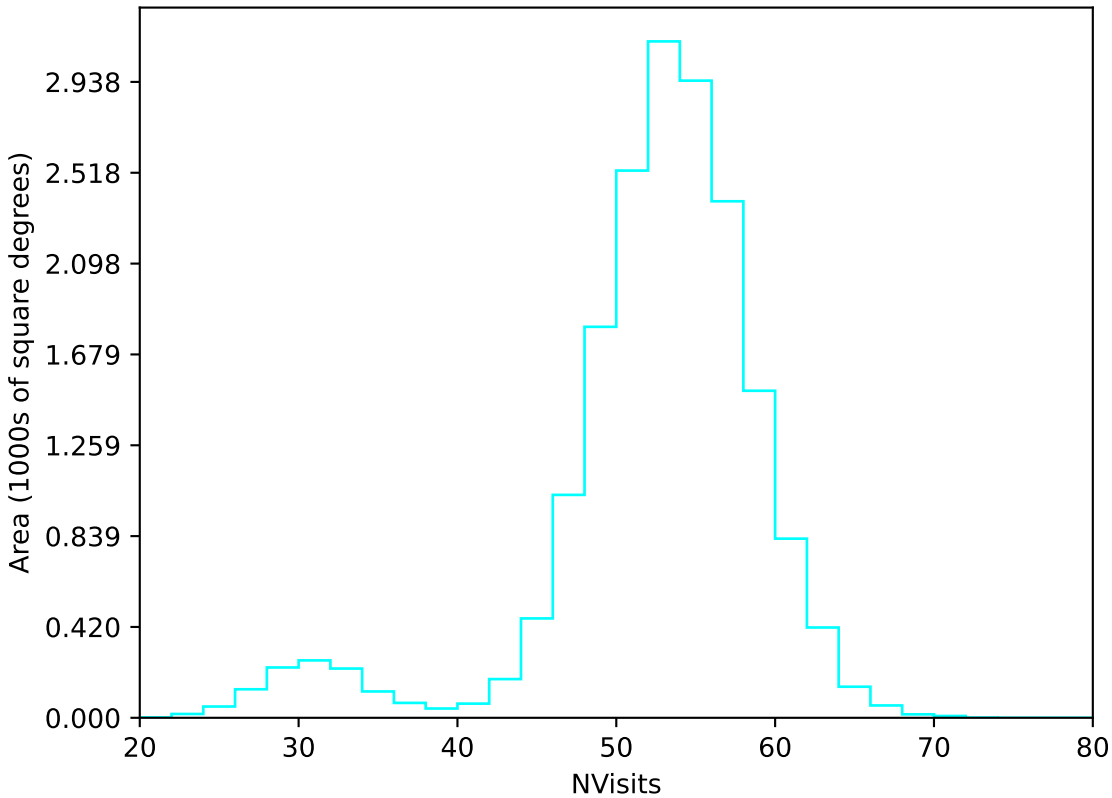
roll_pause_mjdp120_v3.4_10yrs WFD u band: NVisits
