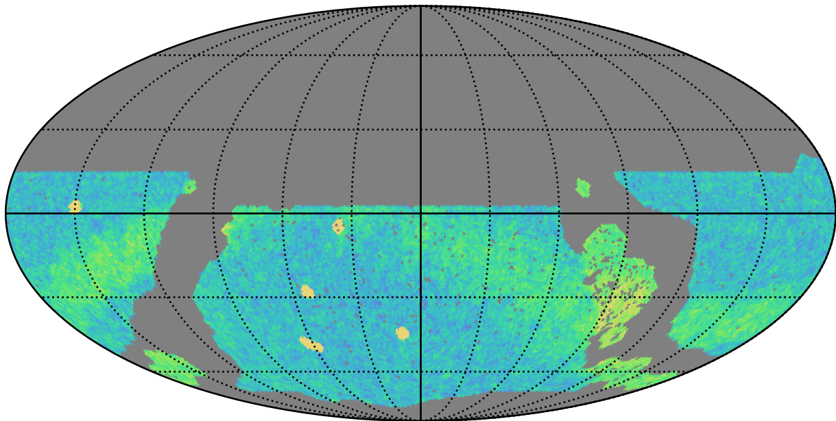
roll_pause_mjdp120_v3.4_10yrs WFD r band: NVisits
